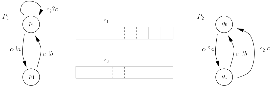
Figure 8: A Communicating Finite State Machine
