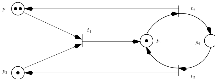
Figure 5: A Petri net
