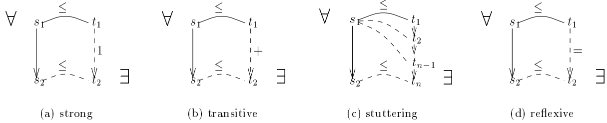
Figure 2: Transitive and stuttering compatibility
