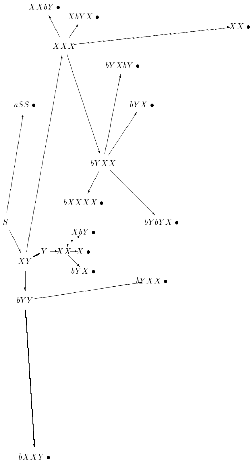
Figure 7: FRT(S) in \langle \mathcal{S}_G, \subseteq \rangle . “•” marks subsumed nodes
