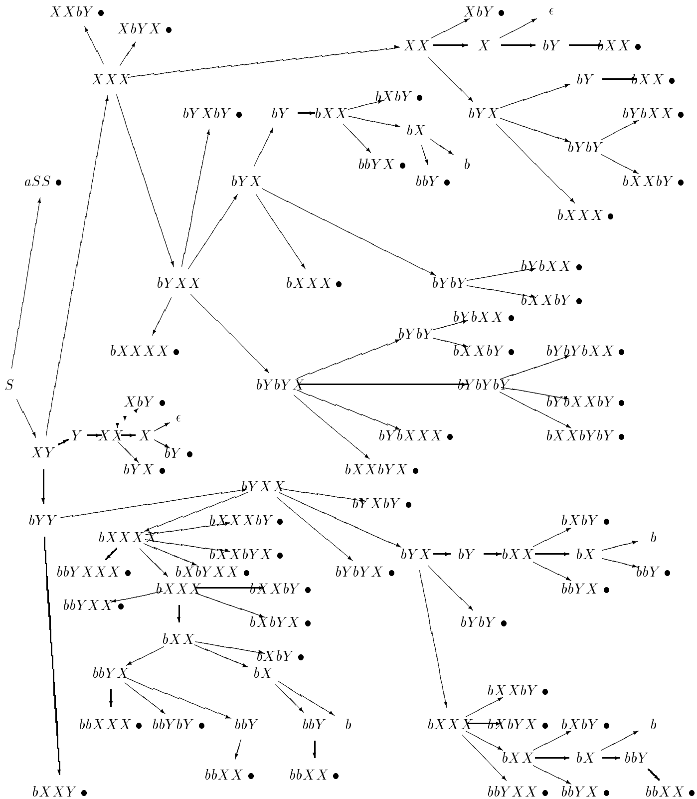
Figure 6: FRT(S) in \langle S_G, \preccurlyeq \rangle . “•” marks subsumed nodes
